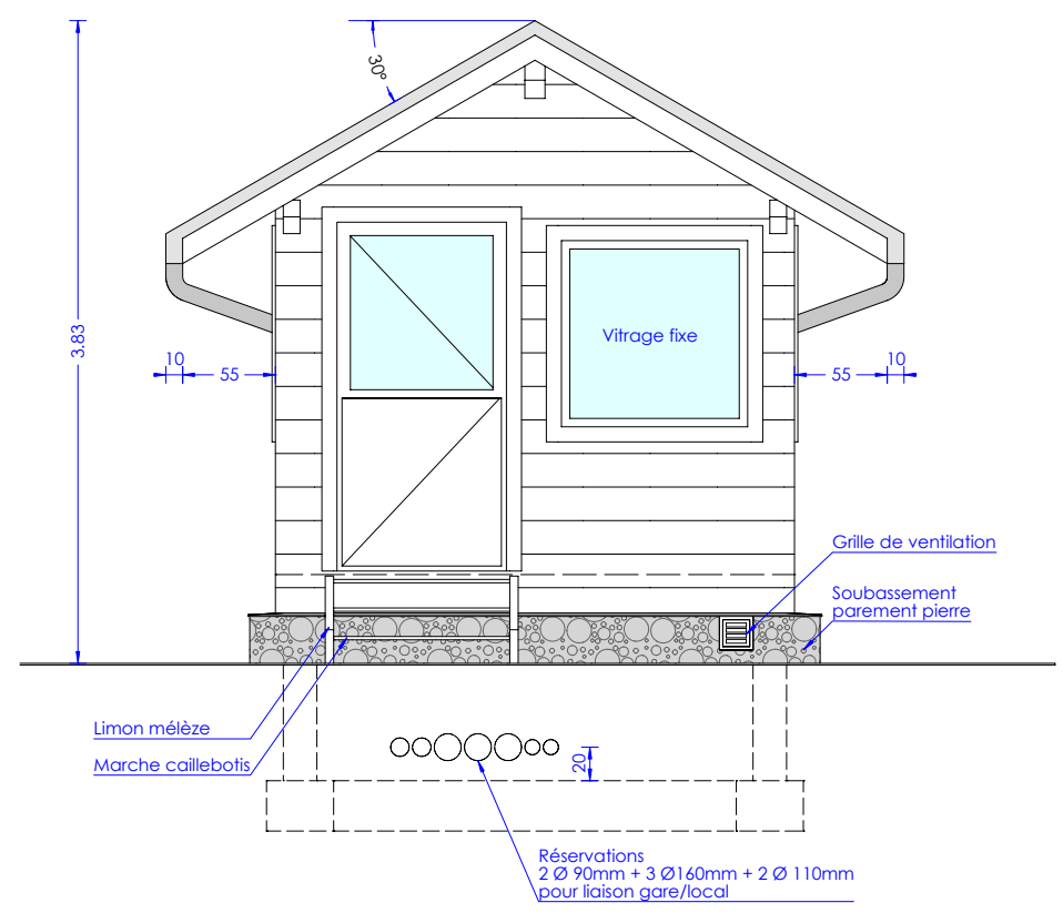
FACADE SUD
