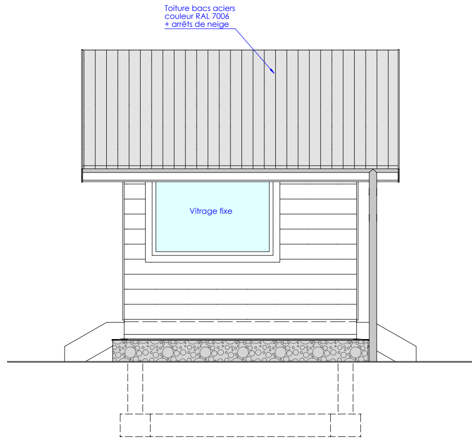
FACADE SUD
